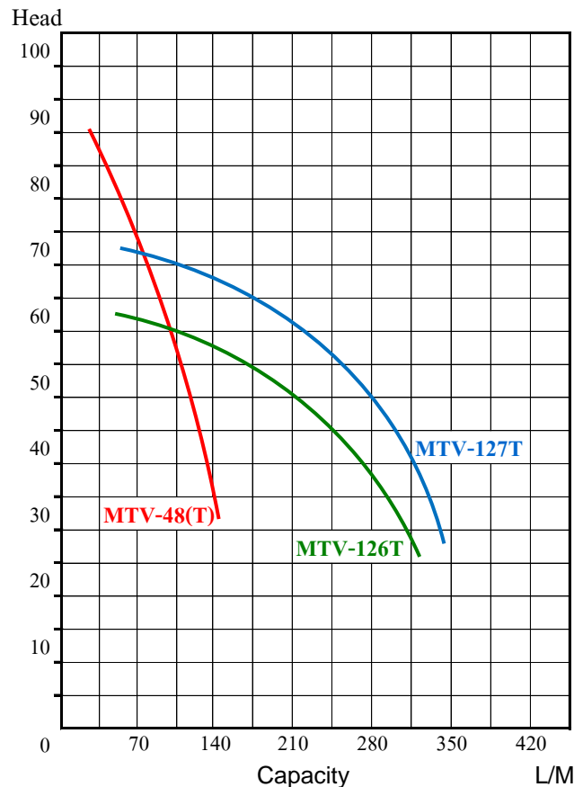
Performance Curve
